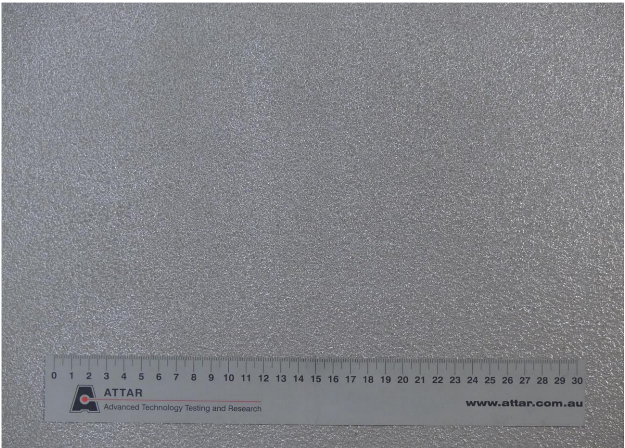
Figure 1: Fosroc Nitoflor FC150 HP + Fosroc Nitoflor Anti-Slip Grains 02 Silica Sand 30/60# + Fosroc Nitoflor FC150 HP
